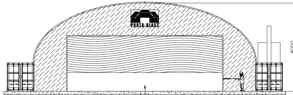
workpiece inlet/outlet FRONT VIEW
