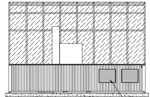
blasting ventilation outlet SIDE VIEW BLASTING
